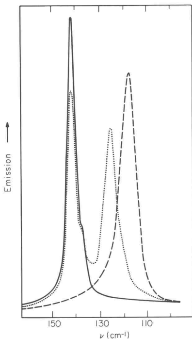
FIG. 11. The spectra of \text{HgI}_2 at various pressures: (---) atmospheric pressure (red phase only), peak at 119 \text{ cm}^{-1} ; ( \cdots ) intermediate pressure (red and yellow phases present), peaks at 126 and 143 \text{ cm}^{-1} and a weak shoulder at 138 \text{ cm}^{-1} ; (—) high pressure (yellow phase only), peak at 143 \text{ cm}^{-1} with a weak shoulder at 138 \text{ cm}^{-1} .
